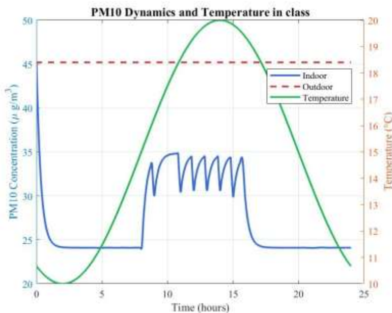
Fig. 4: Simulation results for particulate matter PM 10 and temperature.
