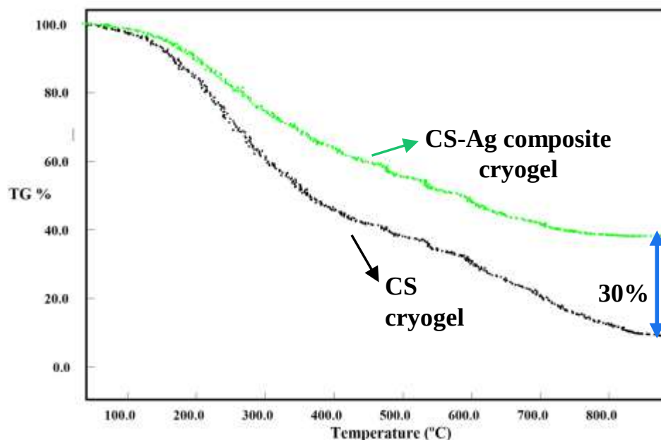
Figure 8. TG% of bare CS cryogel and CS-Ag composite cryogel
