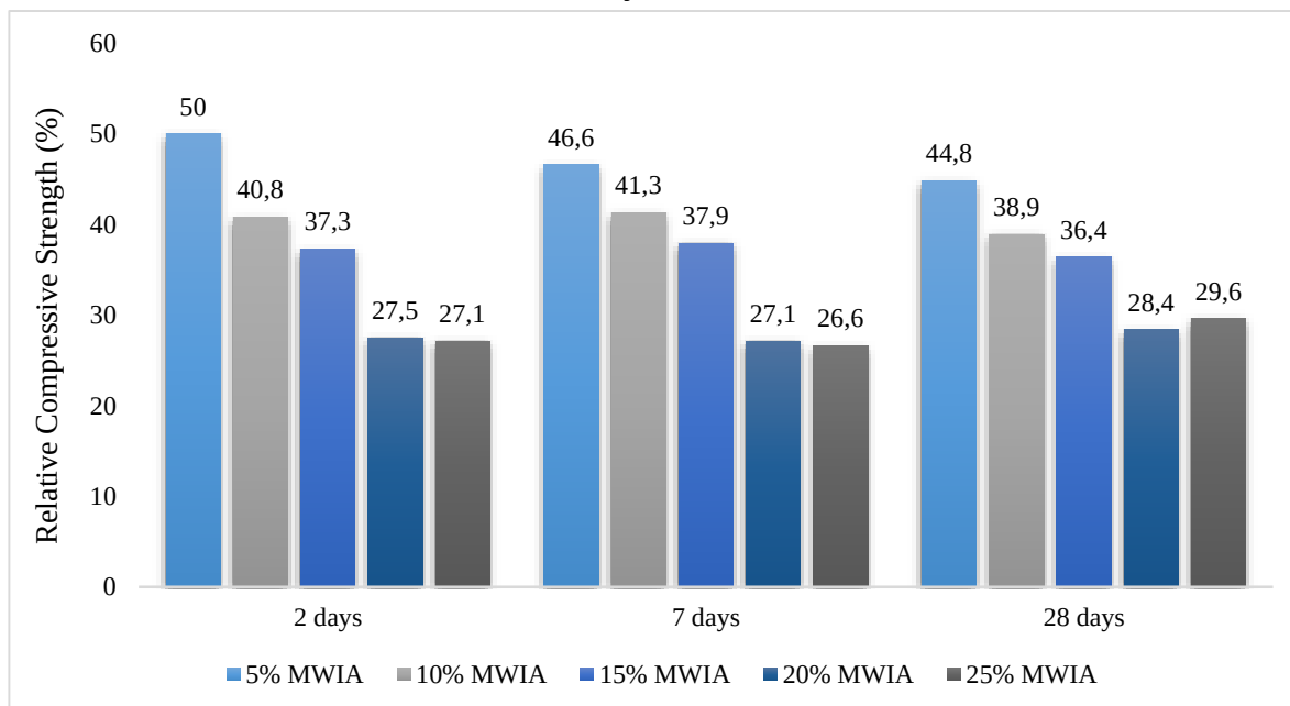
Fig. 10 Relative compressive strength of all samples compared to the control at 2, 7, and 28 days.
