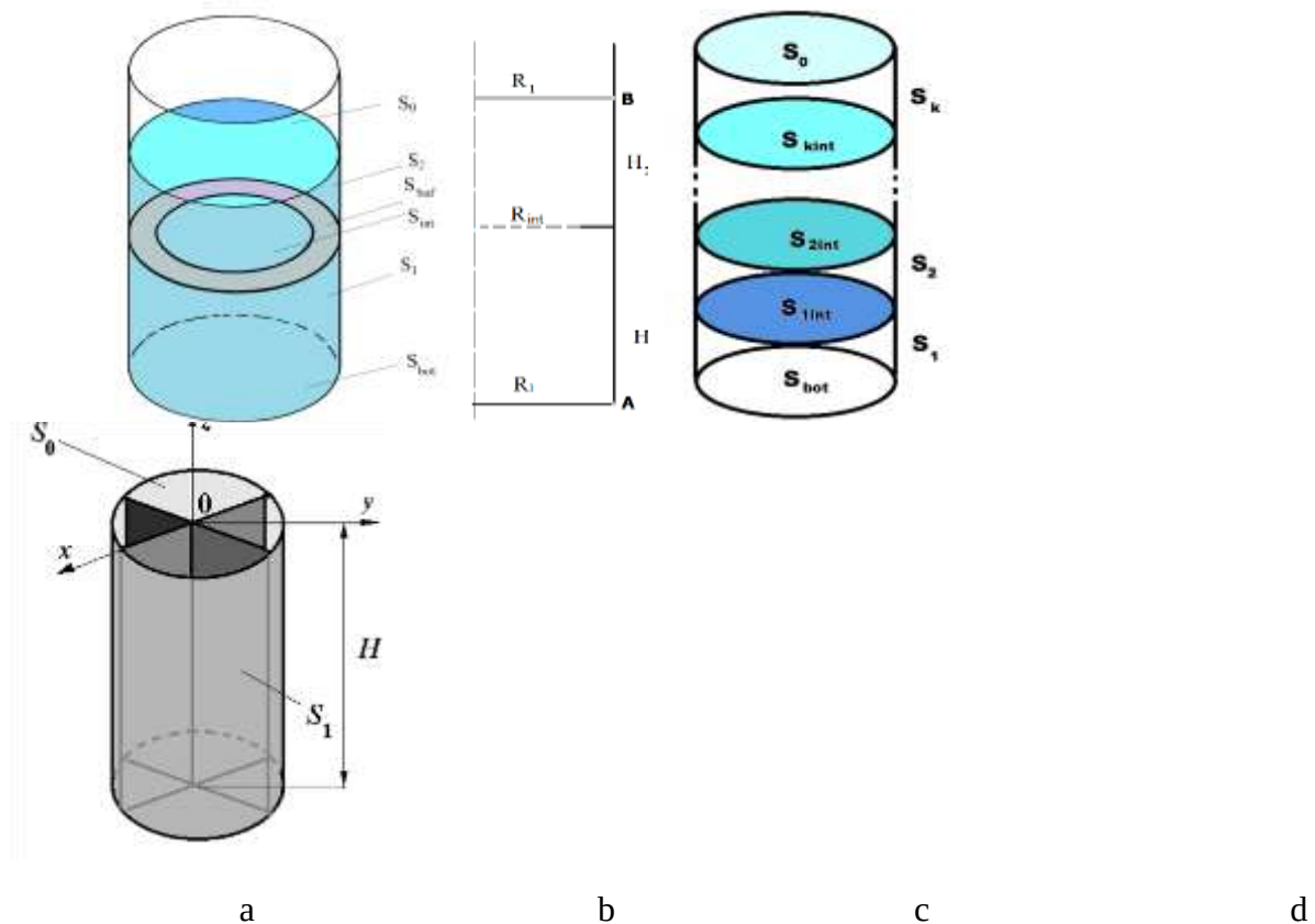
Figure 1. Shells of revolution with baffles.
