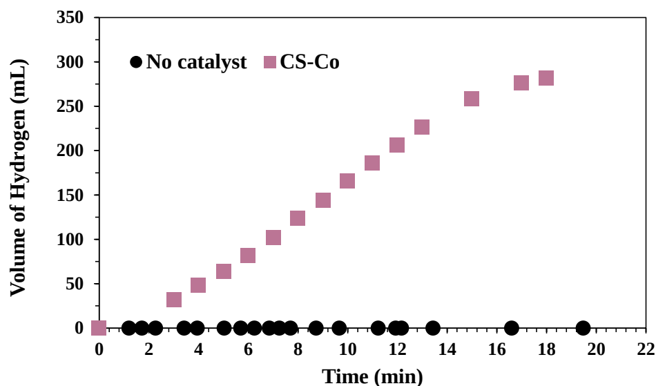
Figure 7. The catalytic effect of CS-Co composite on the hydrolysis of \text{NaBH}_4 [Reaction conditions: 0.280 g composite; 50 mL 50 mM \text{NaBH}_4 at 50 °C with % 5 NaOH, 1000 rpm mixing rate].
