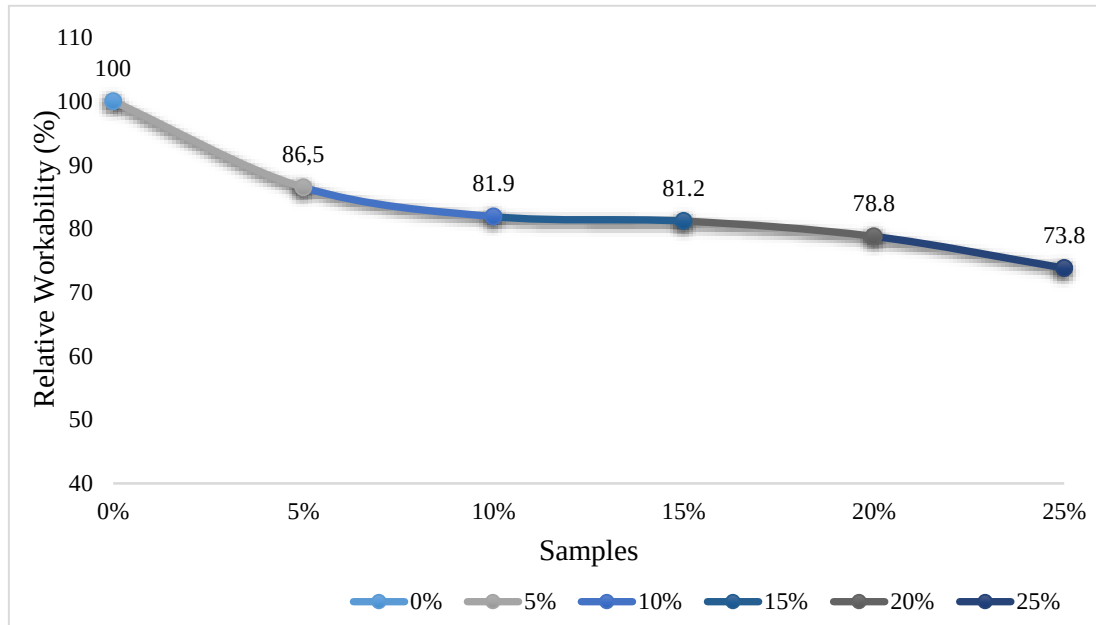
Fig. 7 Relative workability of CEM I 42.5R and the samples containing MWIA.
