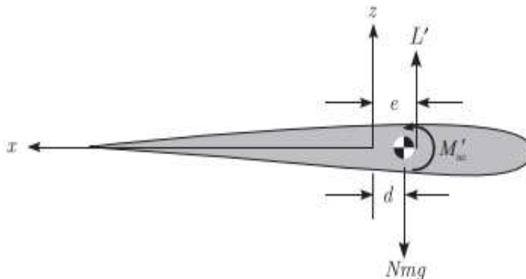
Figure 3 : Uniform unswept clamped-free lifting surface[1]
