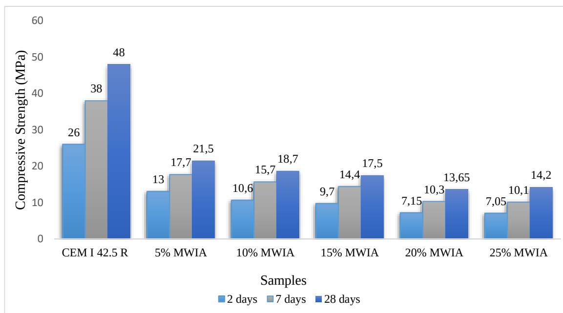
Fig. 9 Compressive strength results for all samples after 2, 7, and 28 days.
