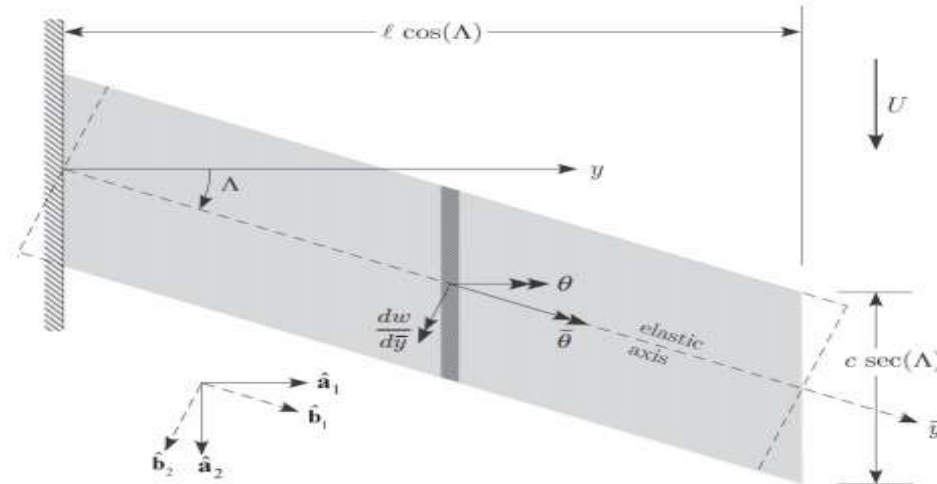
Figure 4 : Schematic of swept wing (positive \Lambda )[1]
