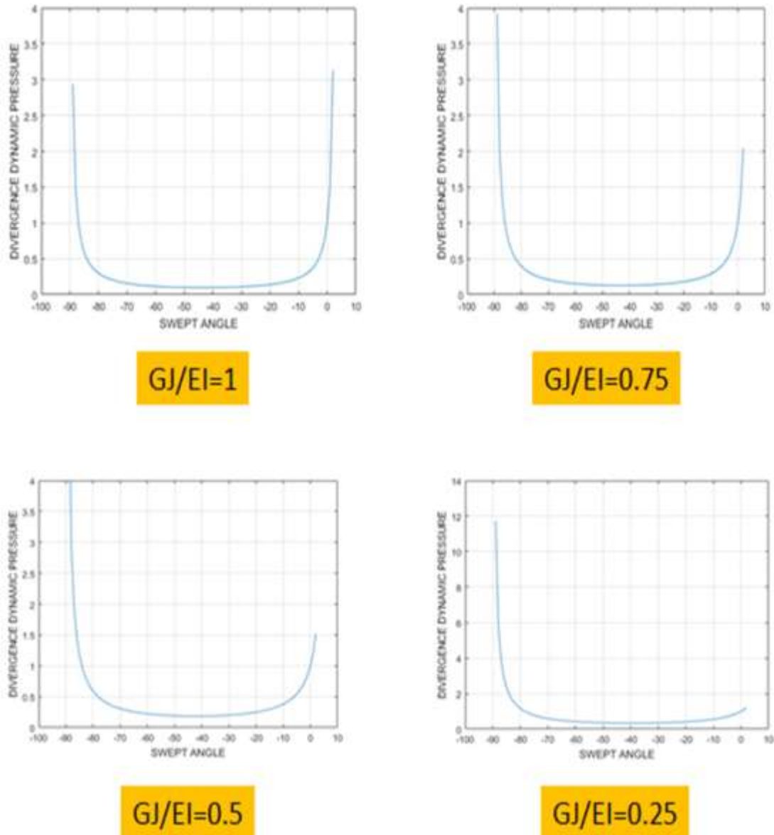
Figure 8 : Divergence dynamic pressure for non tapered swept wing.
