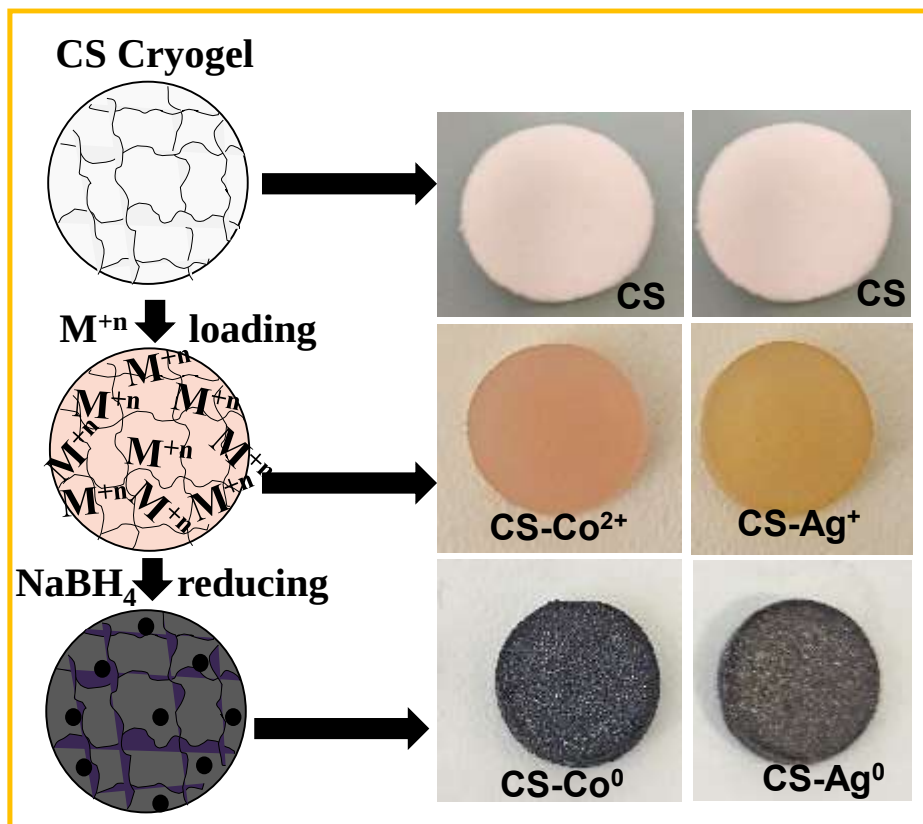
Figure 5. Schematic representation of in situ metal nanoparticles preparation in the CS cryogel network, and their digital camera images.
