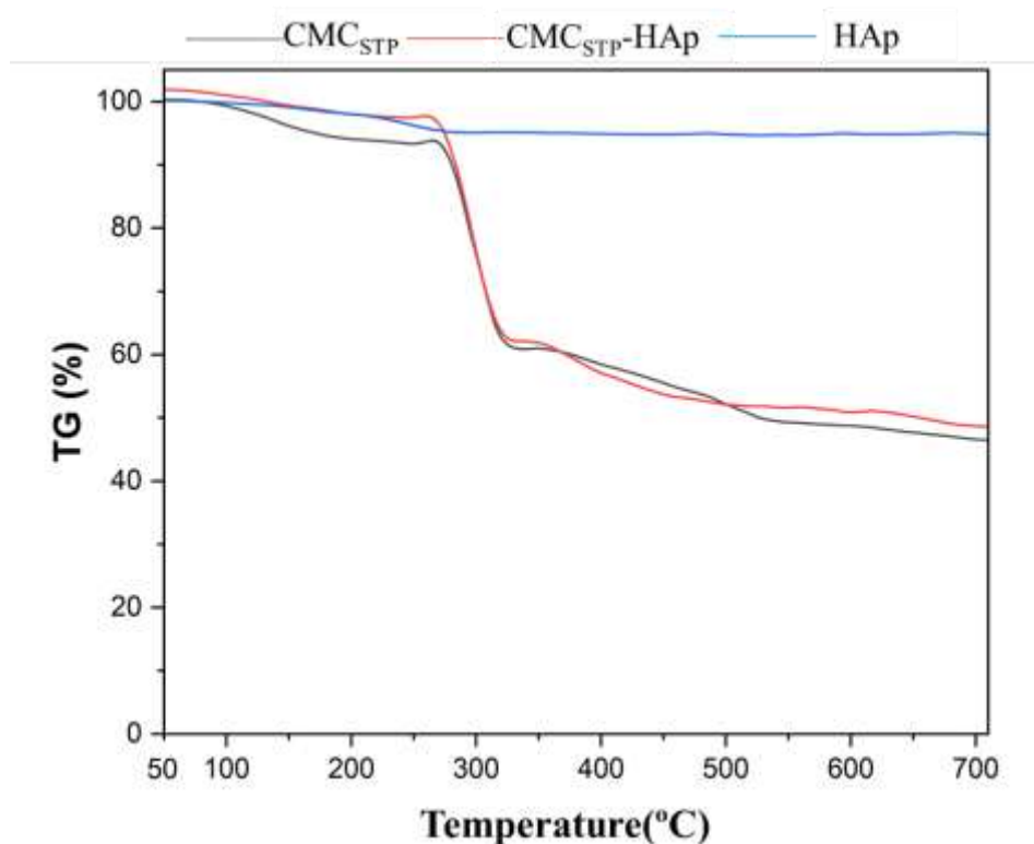
Figure 2. TGA results for CMC STP , CMC STP -HAp and HAp samples.
