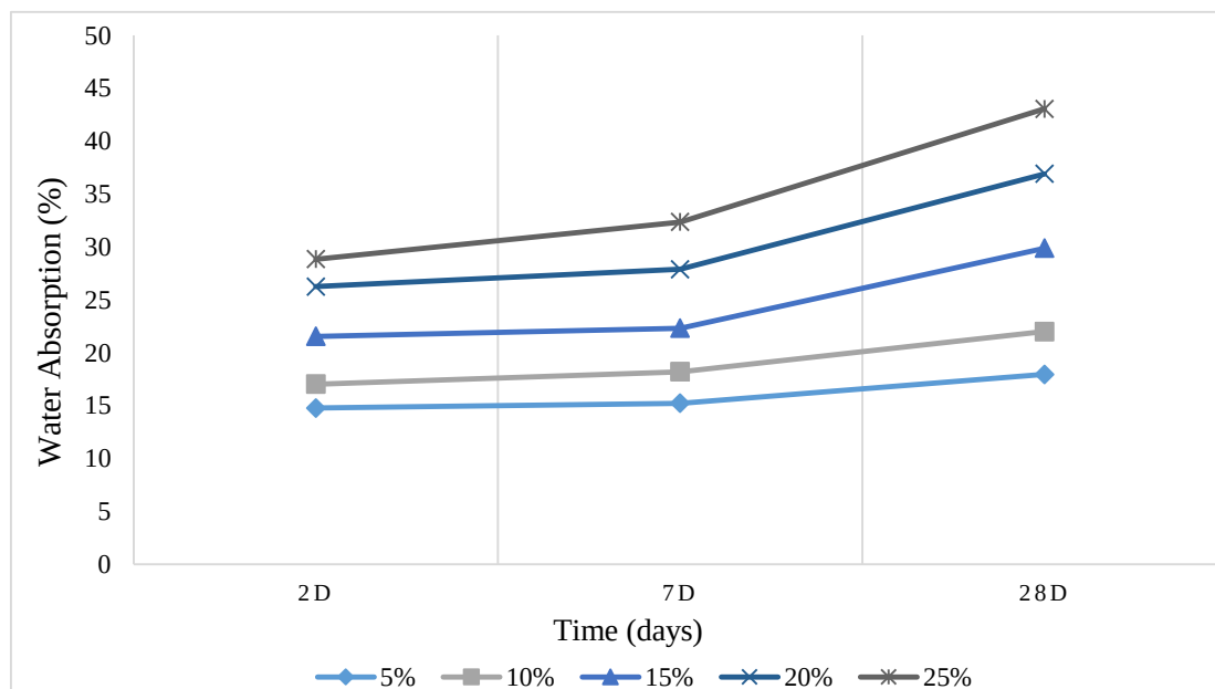
Fig. 8 Water absorption results for all samples after 2,7 and 28 days of immersion in water.
