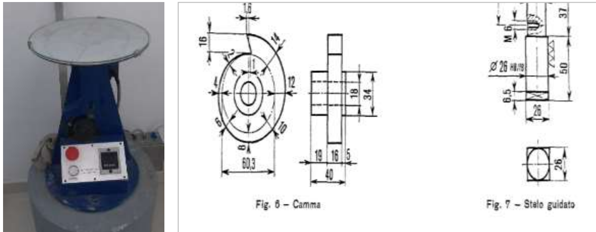
Fig. 4 Workability apparatus and dimensions of the workability testing device.
