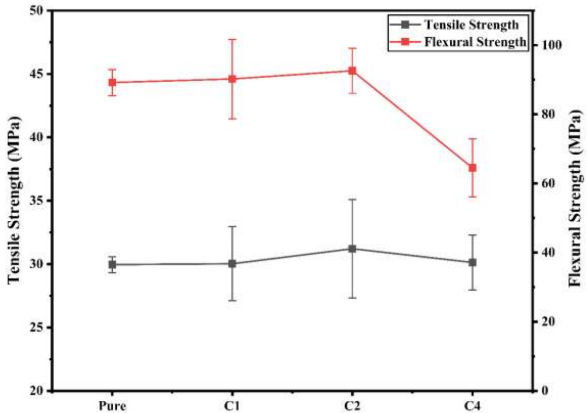
Figure 1. Tensile and flexural strength graphs of pure and composite samples.
