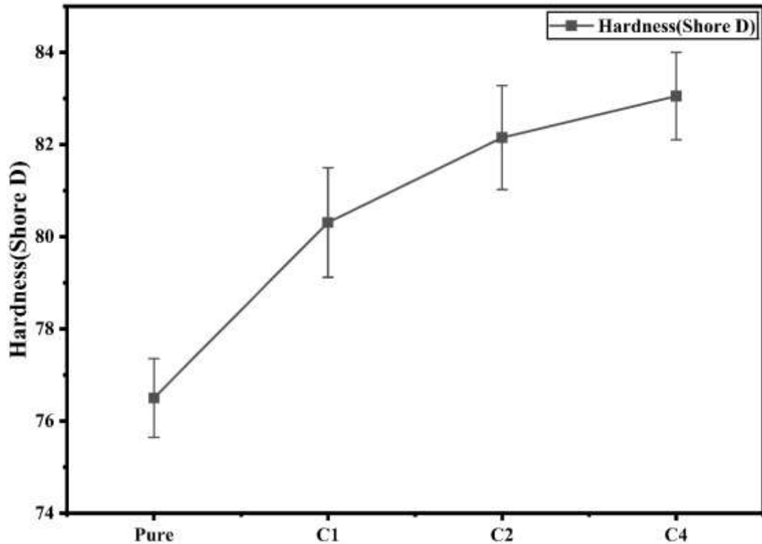
Figure 2. Shore D hardness graph of pure and composite samples.
