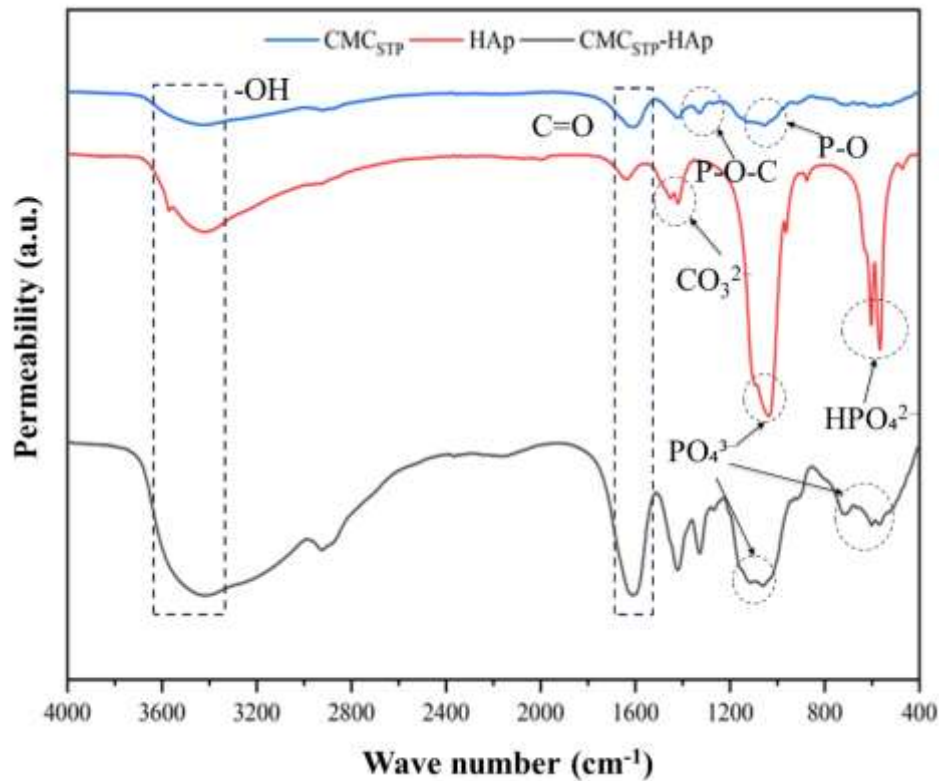
Figure 3. FT-IR spectrum for CMC STP , CMC STP -HAp and HAp samples
