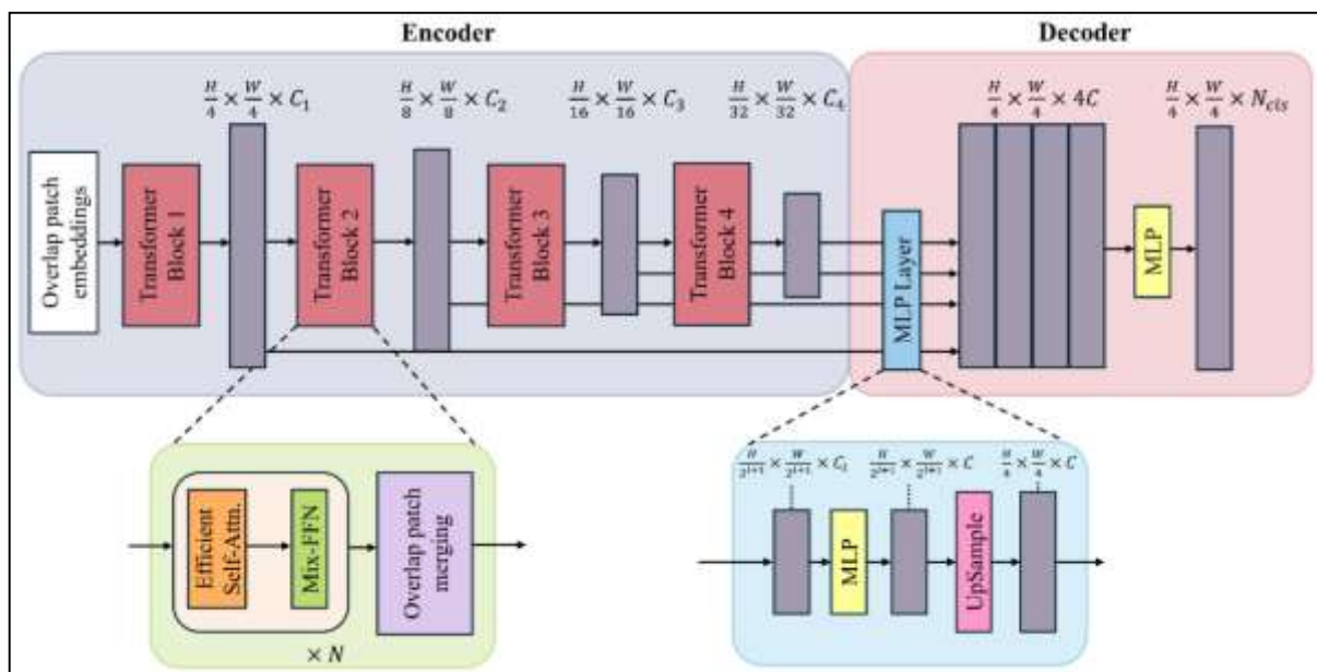
Figure 2. Architecture of the SegFormer.
