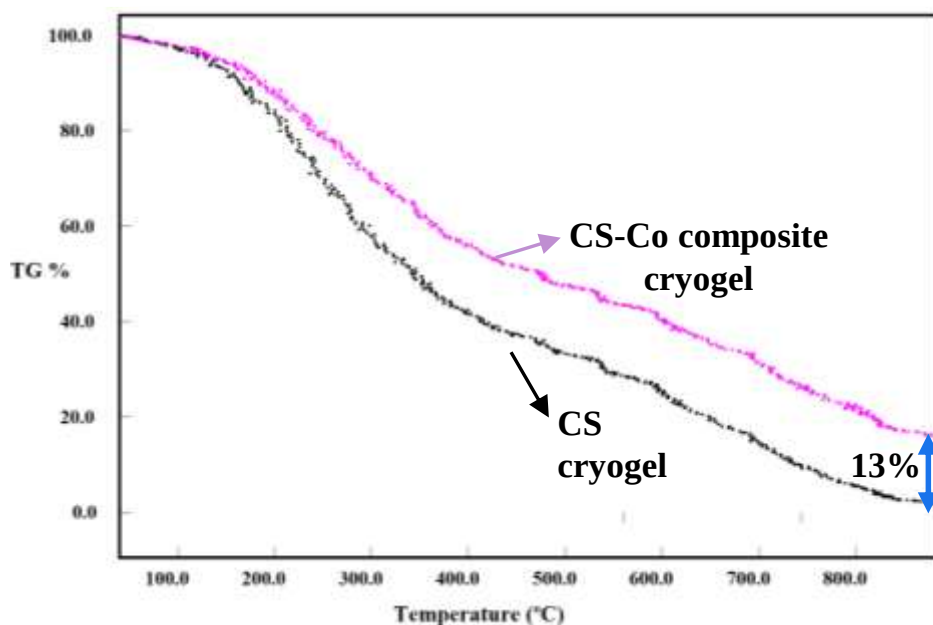
Figure 6. TG% of bare CS cryogel and CS-Co composite cryogel.
