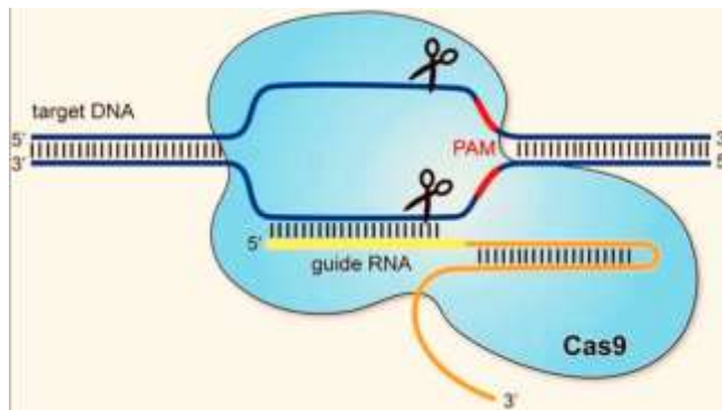
Figure 3. Schematic drawing of a Clustered regularly interspaced palindromic repeats (CRISPR)
