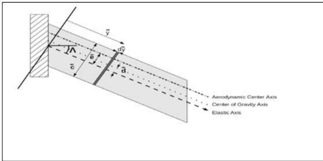
Figure 7 : Non tapered swept wing(model 1).
