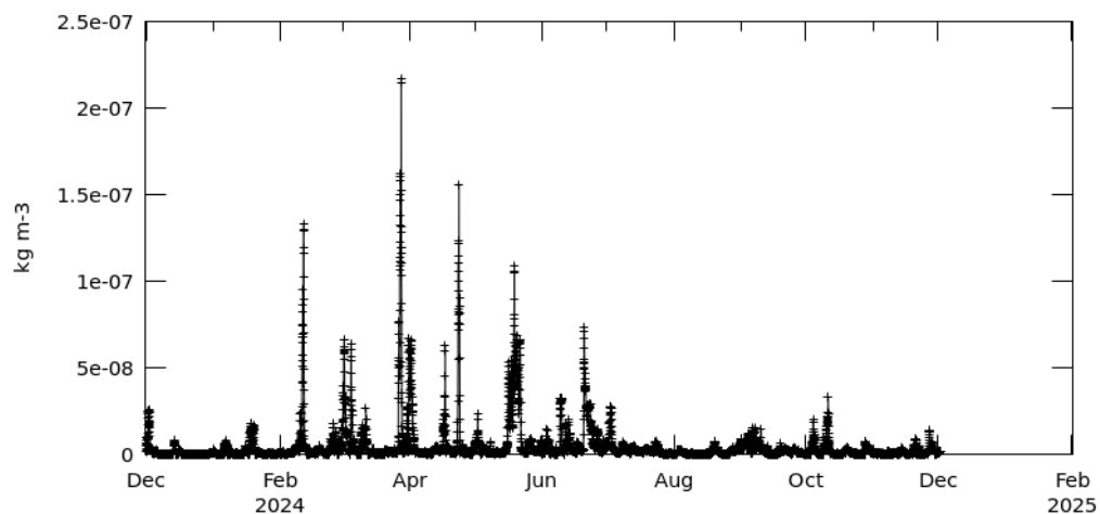
Fig.1 Time series from model MERRA 2 for hourly concentration of PM 2.5 in Tirana during 2023-12-01 to 2024-12-01.
