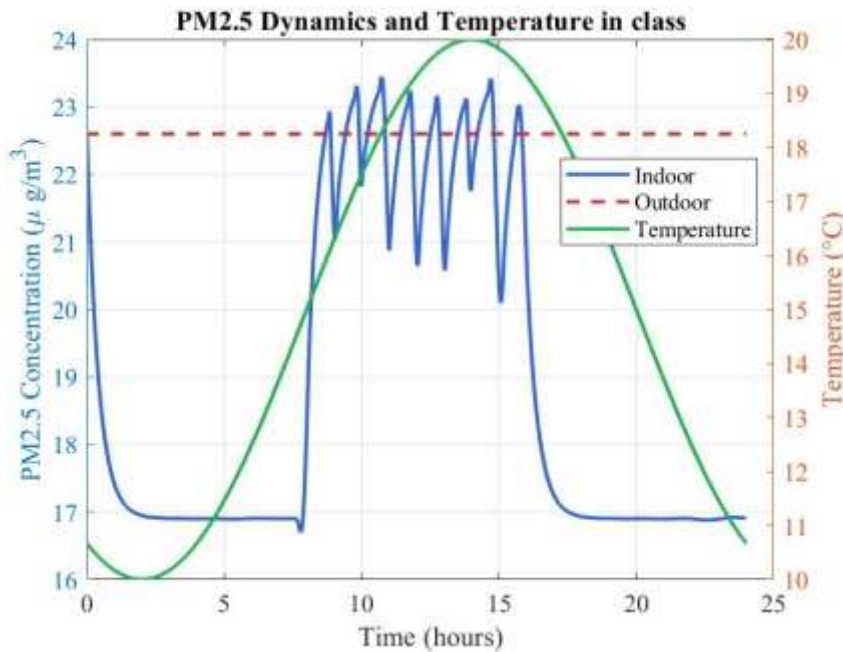
Fig. 3. Simulation results for particulate matter PM 2.5 and temperature.
