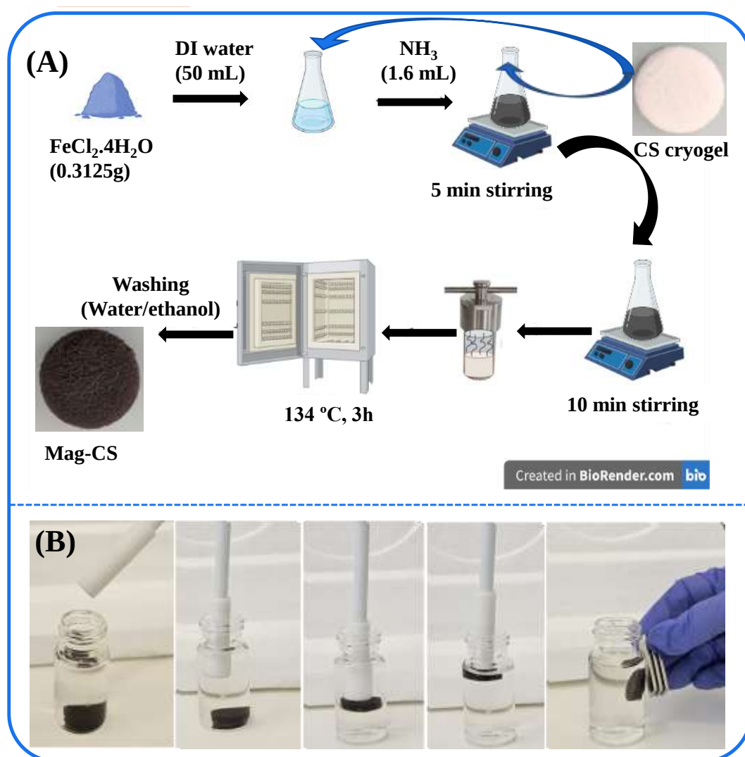
Figure 3. Hydrothermally supported mag-CS cryogel synthesis scheme and digital camera images of mag-CS subjected to a magnetic field.
