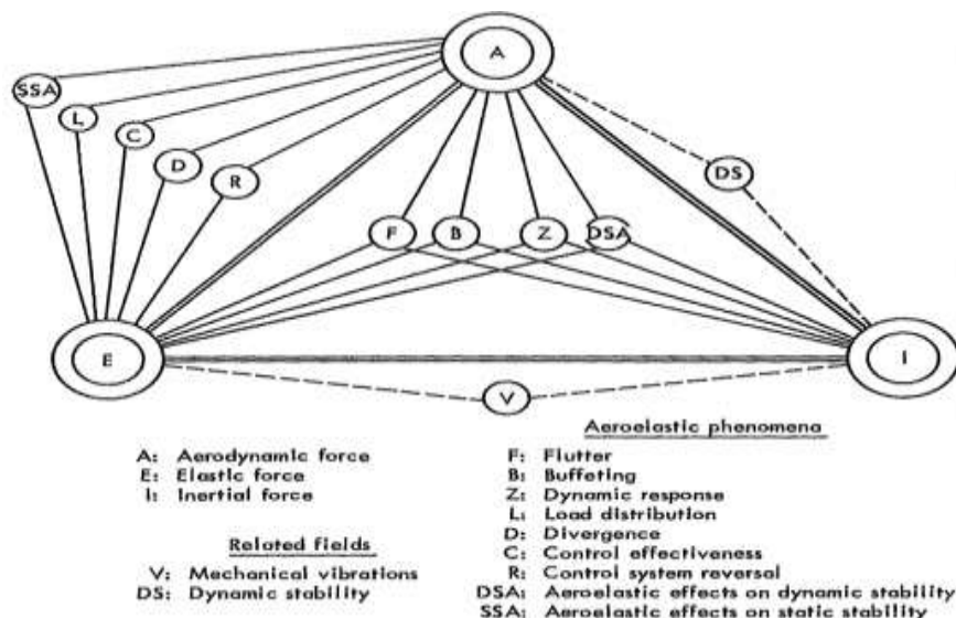
Figure 1: The aeroelastic triangle of forces.[4]
